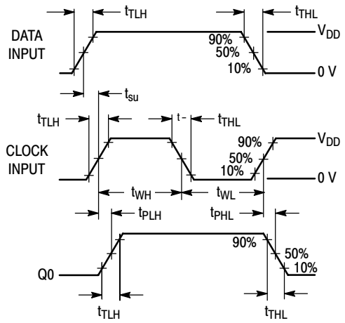
Figure 2. Switching Test Circuit and Waveforms
