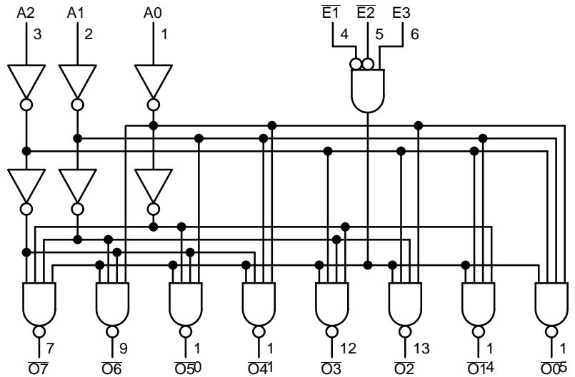
Figure 2. Logic Diagram
