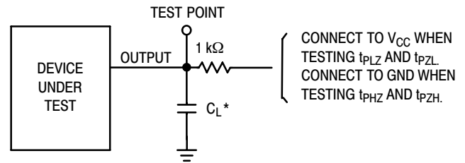
Figure 7. Test Circuit
