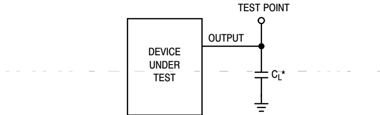
Figure 5. Test Circuit
