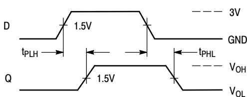
Figure 3. Switching Waveform
