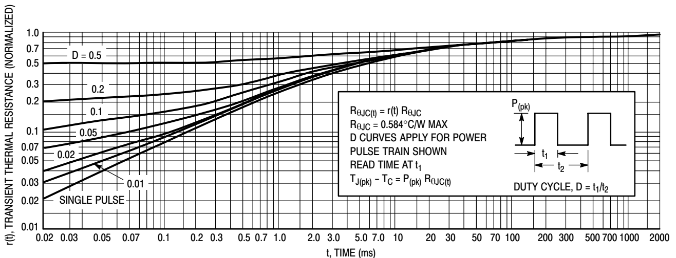
Figure 13. Thermal Response
