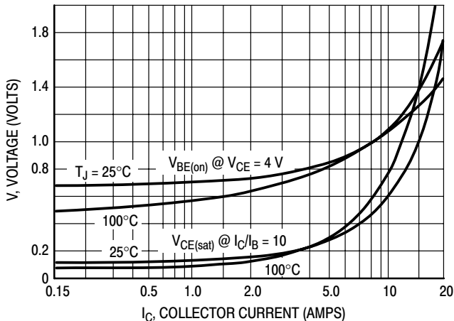
Figure 5. "On" Voltage
