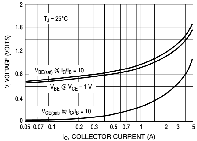
Figure 6. "On" Voltage
