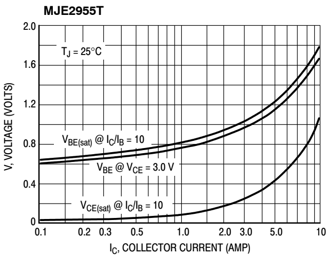
Figure 4. "On" Voltages
