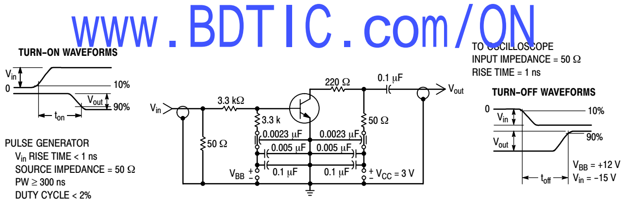
Figure 5. Turn-On and Turn-Off Time Test Circuit
