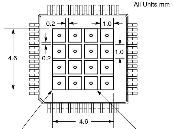
Figure 9. Recommended Solder Mask Openings
