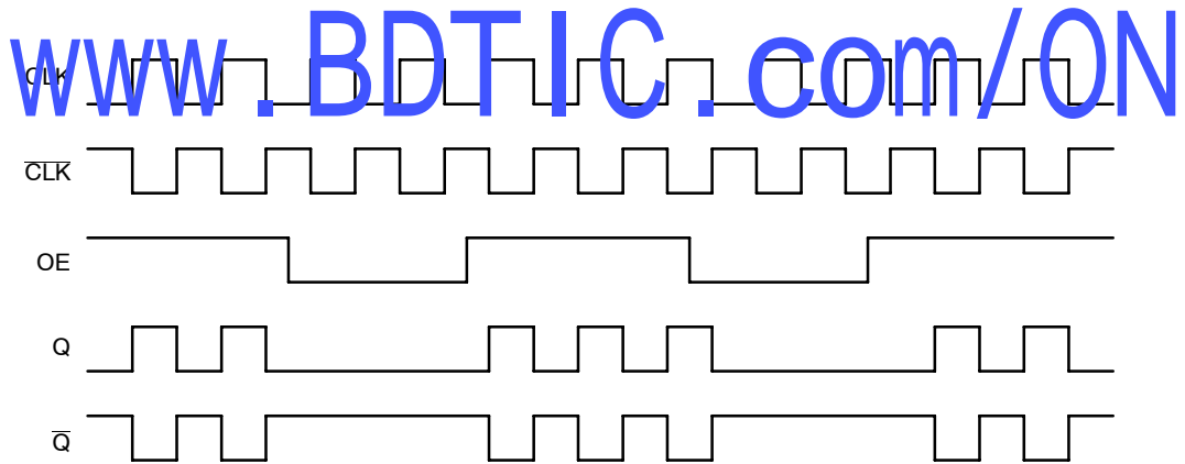
Figure 7. Output Enable (OE) Timing Diagram
