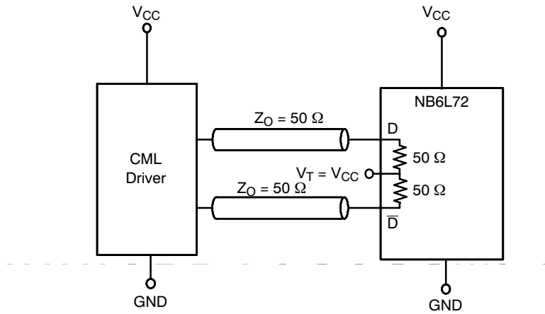
Figure 12. Standard 50\ \Omega Load CML Interface
