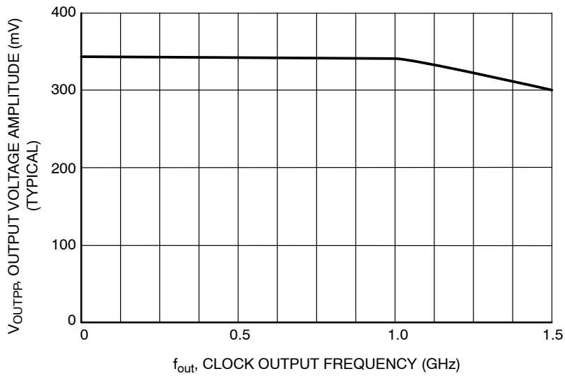
Figure 18. Output Voltage Amplitude (V OUTPP ) versus Output Clock Frequency at 25°C (Typical) f_{out} (QA/QB) = f_{in} \div n ; For n = 2, 4, 8, 16; f in ≤ 3.0 GHz For n = 1; f in ≤ 1.5 GHz
