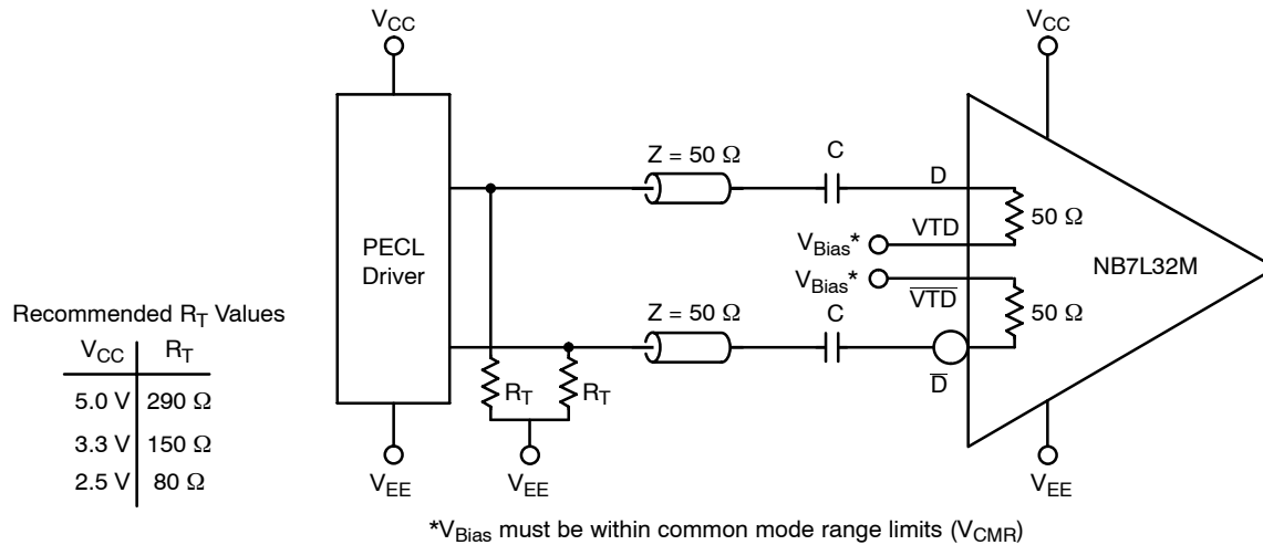
Figure 16. PECL to NB7L32M Interface
