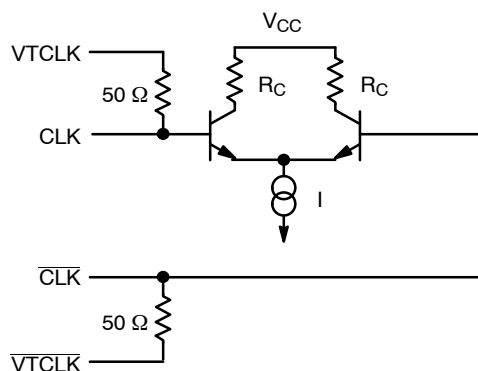
Figure 4. Input Structure
