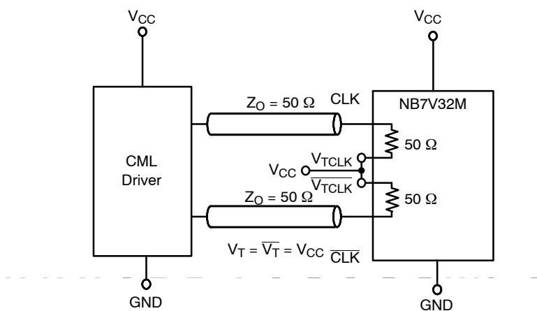
Figure 14. Standard 50 \Omega Load CML Interface
