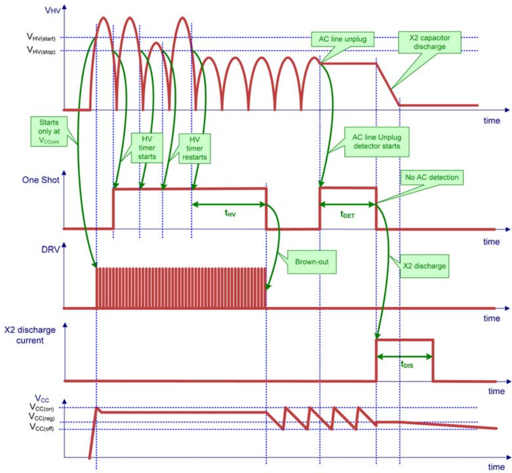
Figure 53. HV Pin ac Input Timing Diagram with X2 Capacitor Discharge Sequence When the Application is Unplugged Under Extremely Low Line Condition
