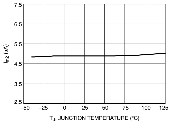
Figure 19. Multiplier Output Current ( V_{control} = V_{CONTROL(max)} , V_{bo} = 0.9\text{ V} , I_{CS} = 75\text{ }\mu\text{A} ) vs. Temperature
