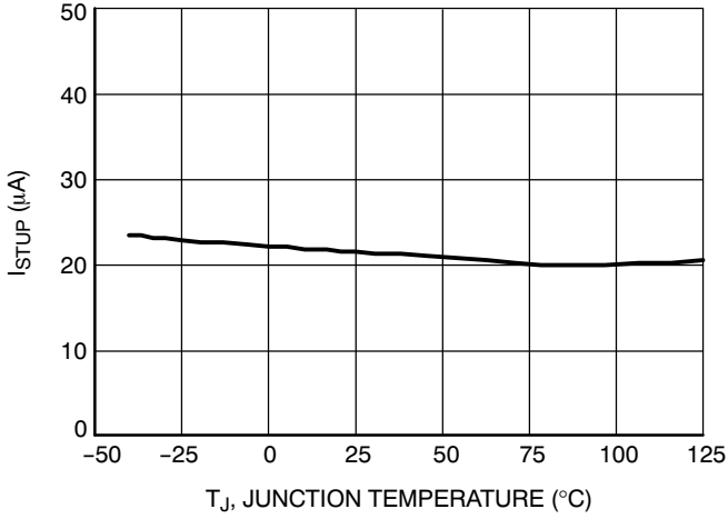
Figure 26. Supply Current in Startup Mode vs. Temperature
