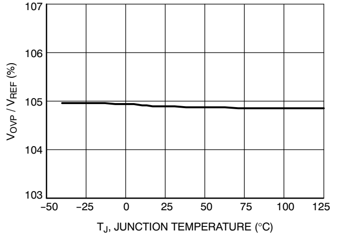
Figure 21. Ratio (Over Voltage Threshold / V REF ) vs. Temperature
