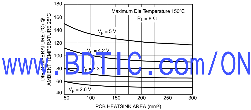
Figure 29. Maximum Die Temperature versus PCB Heatsink Area
