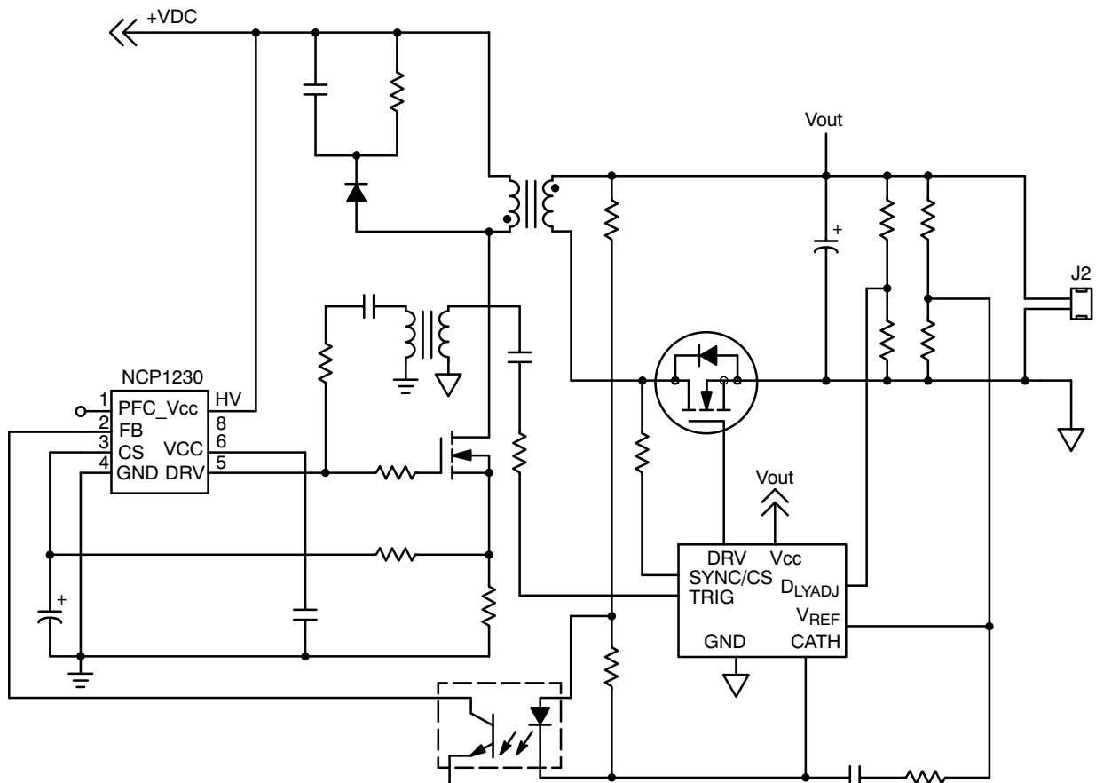
Figure 2. Typical Application
