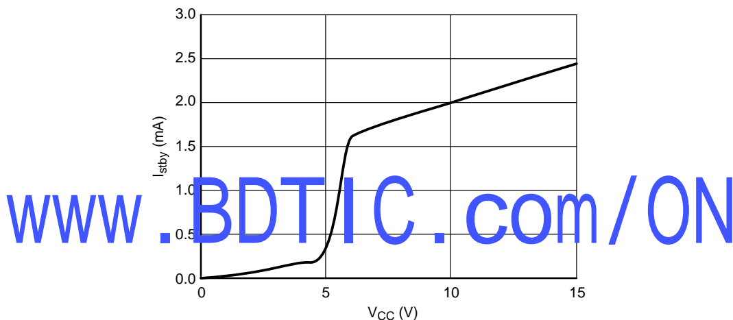
Figure 36. Power Supply Current in Standby Mode vs. Power Supply Voltage – V CC
