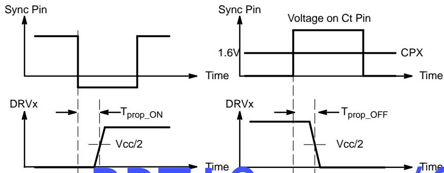
Figure 8. T_{prop\_ON} and T_{prop\_OFF} Propagation Delay Definition (in Normal Mode Operation)
