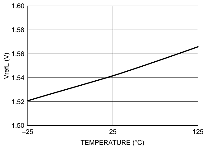
Figure 13. Ramp Control Reference Voltage vs. Temperature (V pin4 falling)
