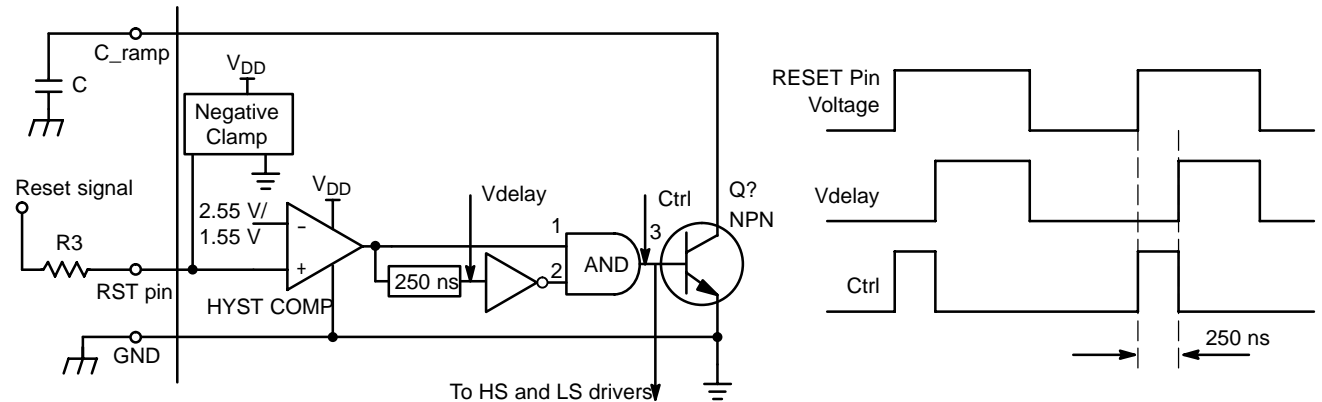
Figure 27. Reset Block
