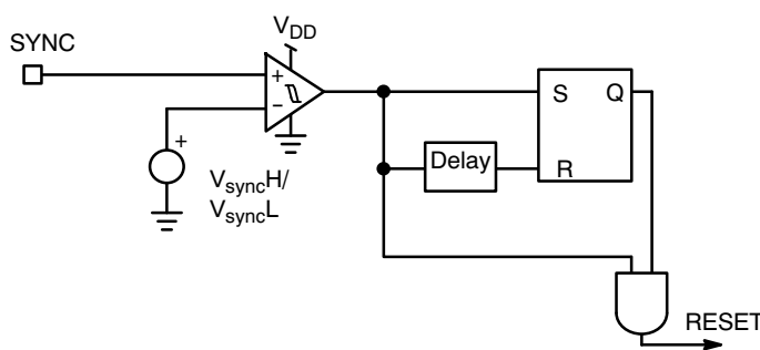
Figure 24. Synchronization Block
