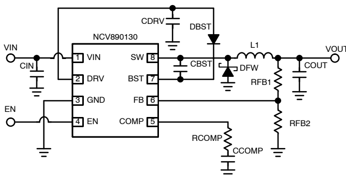
Figure 1. Typical Application
