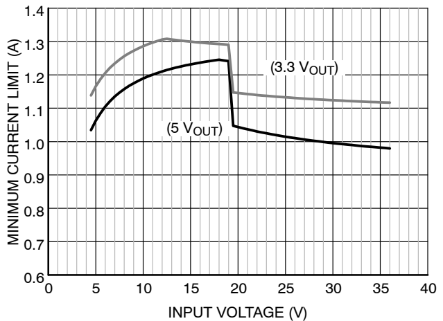
Figure 26. NCV890130 Load Current Capability with 4.7 \mu H Inductor
