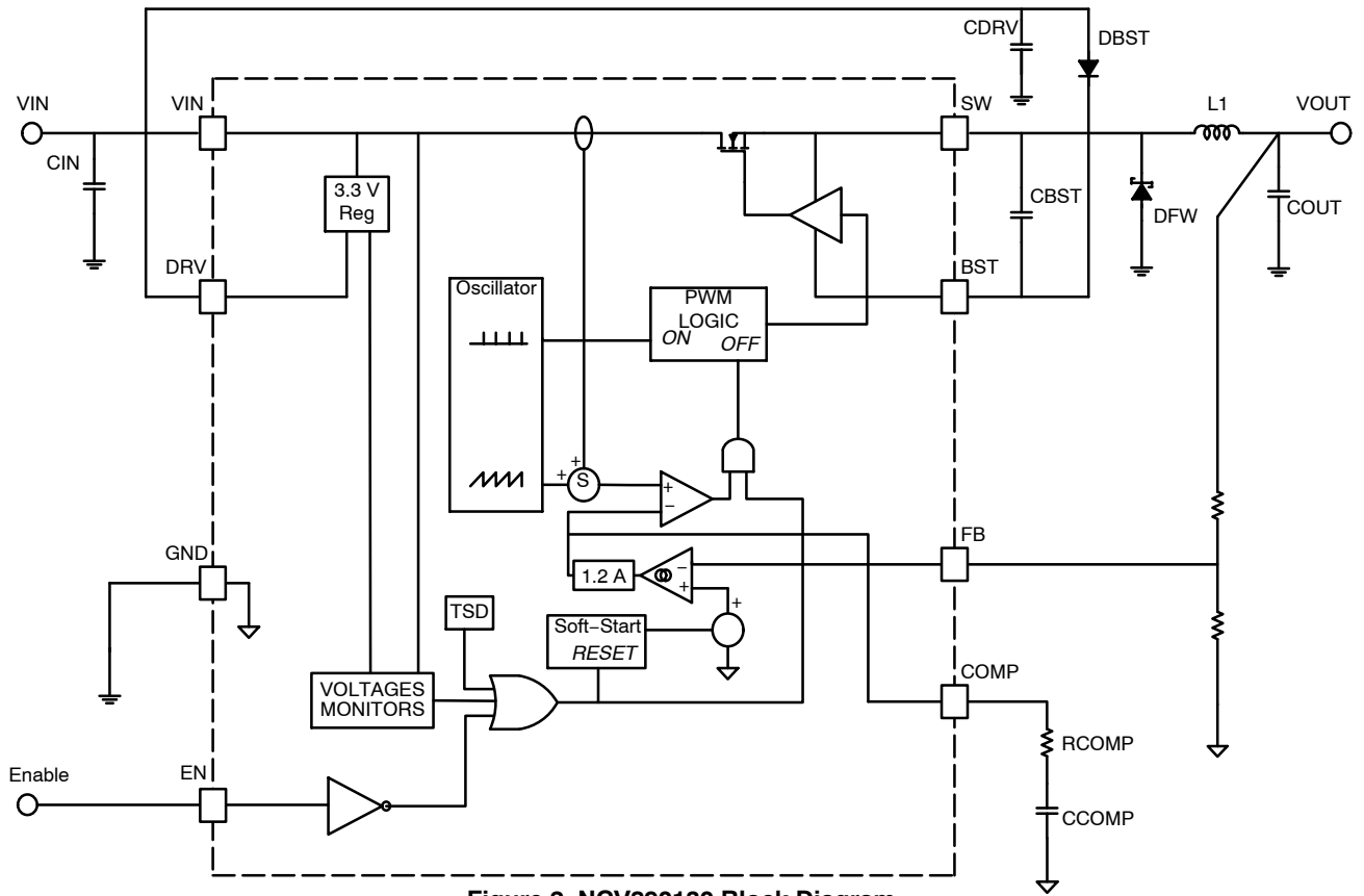
Figure 2. NCV890130 Block Diagram
