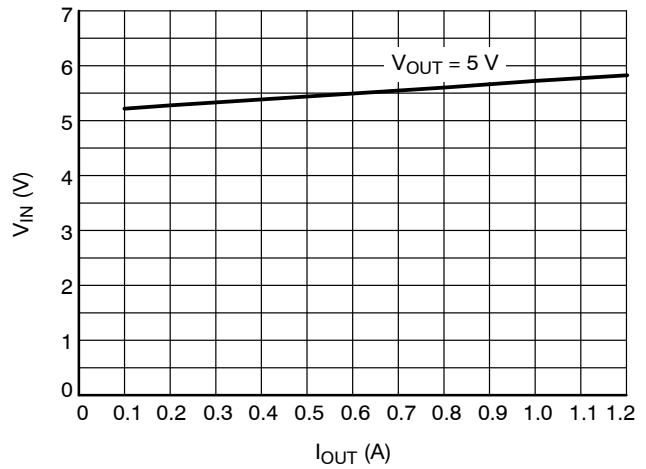
Figure 27. Minimum Input Voltage vs. Output Current
