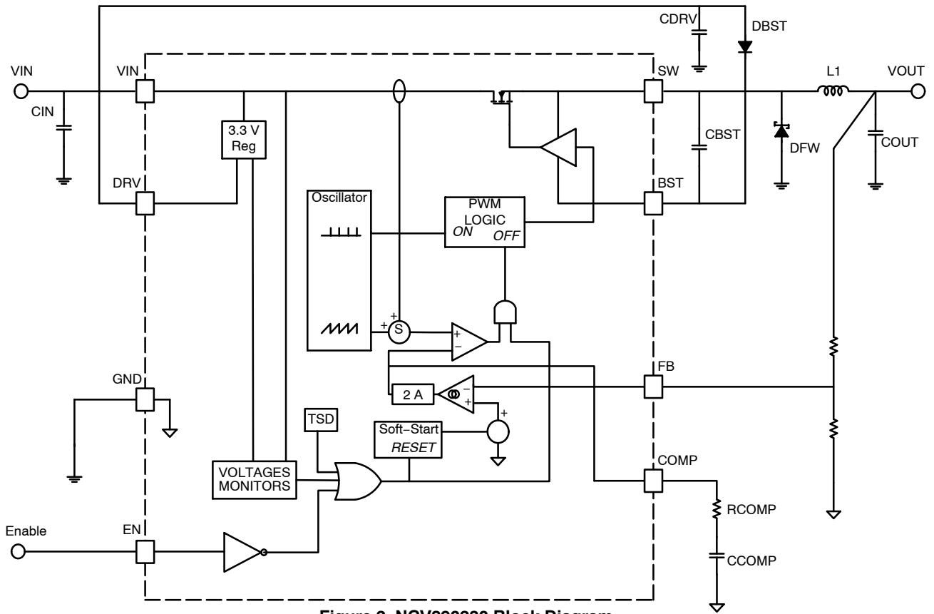
Figure 2. NCV890230 Block Diagram
