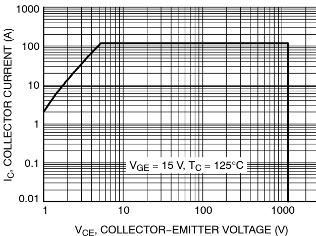
Figure 18. Reverse Bias Safe Operating Area
