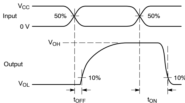
Figure 5. t_{ON}/t_{OFF}
