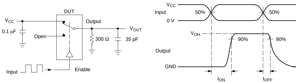
Figure 20. t_{\text{ON}}/t_{\text{OFF}}
