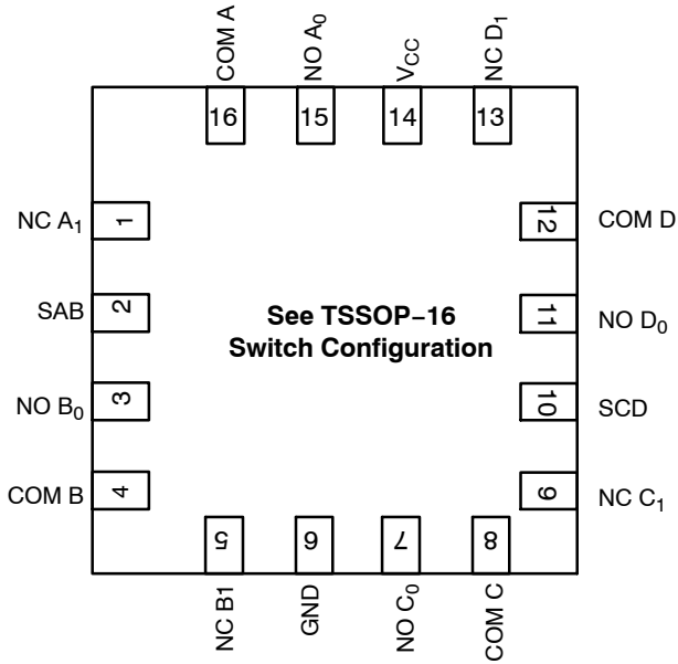
QFN-16 PACKAGE
