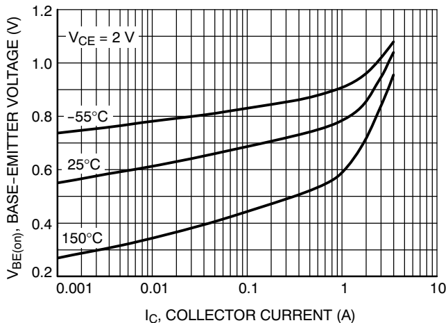
Figure 8. Base-Emitter Voltage
