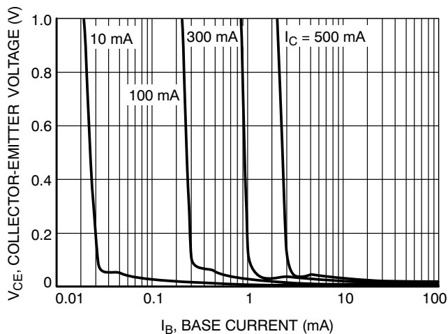
Figure 6. Saturation Region
