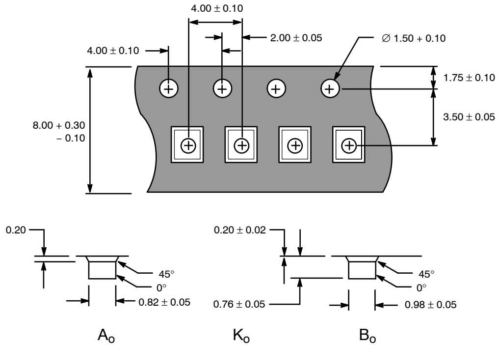
Figure 10. 8 Pillar WLCSP Carrier Tape Drawing
