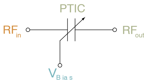
Figure 1. PTIC Functional Block Diagram
