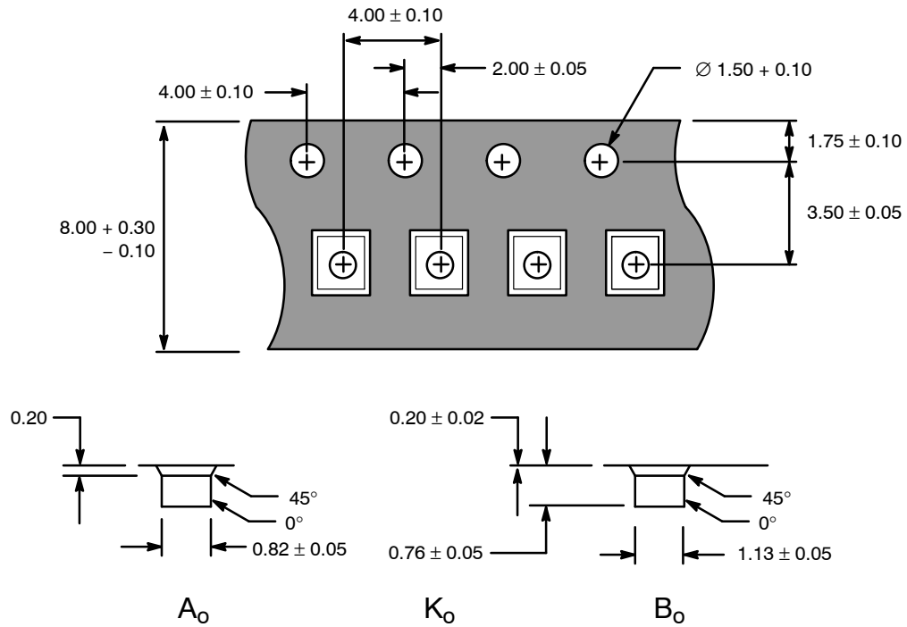
Figure 10. 10 Pillar WLCSP Carrier Tape Drawing
