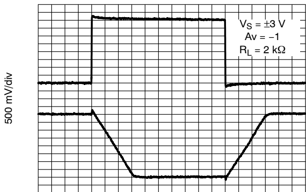
Figure 27. 6 V Inverting Large Signal Pulse Response
