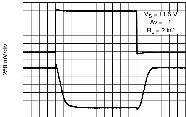
Figure 23. 3 V Inverting Large Signal Pulse Response
