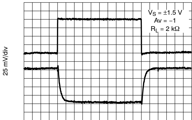
Figure 25. 3 V Inverting Small Signal Pulse Response
