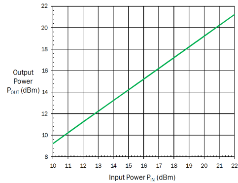
Output Power versus Input Power (Temperature=25°C, VRF=2.6V)
