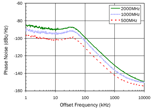
VC02 With Passive Loop Filter
