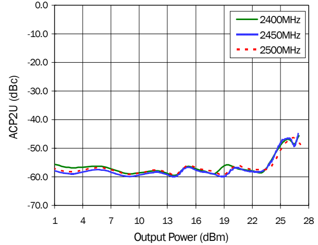
ACP2 (Upper) versus Output Power over Frequency
