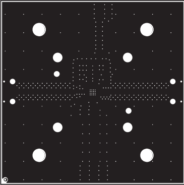
Inner 2
