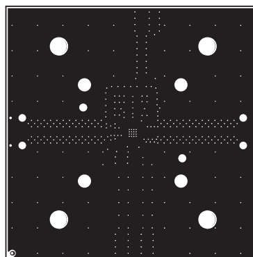
Inner 2
