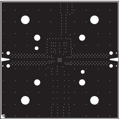
Inner 1
