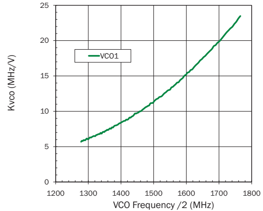
VC01 Frequency versus Kvco LO Divide by 2
