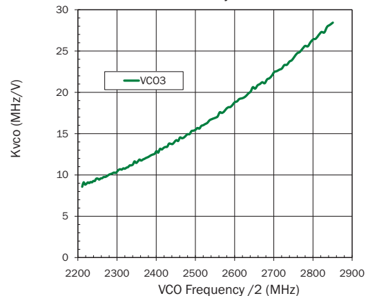
VC03 Frequency versus Kvco LO Divide by 2
