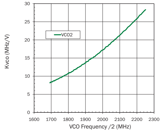
VC02 Frequency versus Kvco LO Divide by 2
