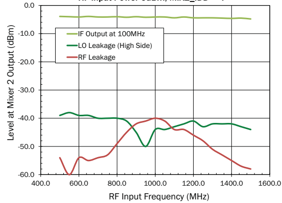
LO & RF Leakage at Mixer 2 Output RF Input Power 0dBm, MIX2_IDD = 4
