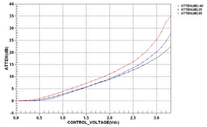
ATTENUATION VS. CONTROL VOLTAGE VS. TEMPERATURE @ 2350 MHz
