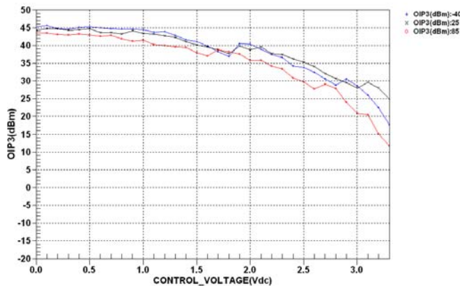
OUTPUT IP3 VS. CONTROL VOLTAGE VS. TEMPERATURE @ 2350 MHz
