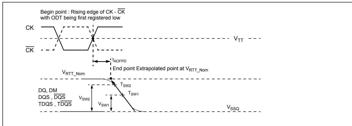
Figure 17. Definition of tAOPFD
