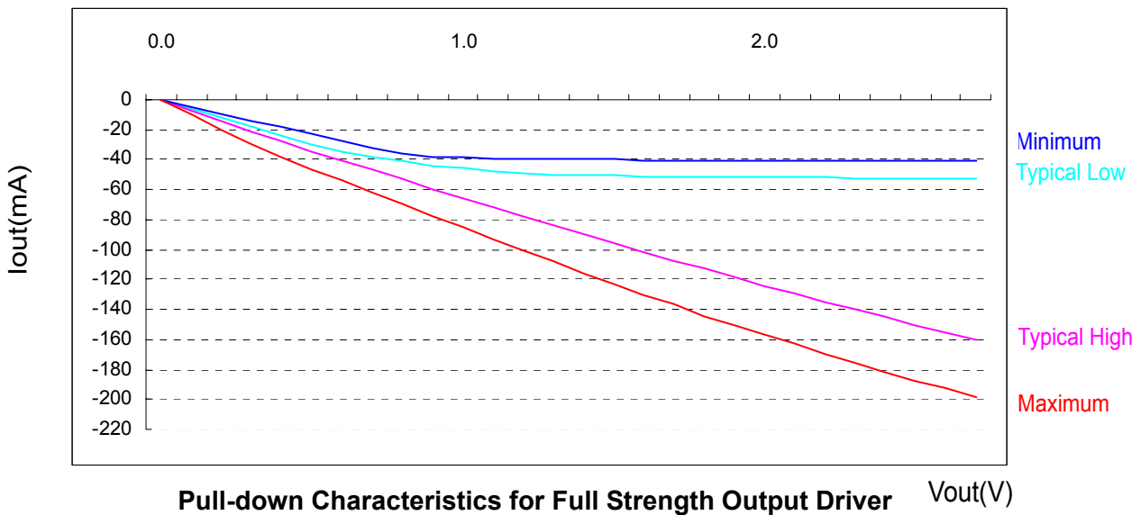
Figure 4. I/V Characteristics for input/output buffers : Pull up(above) and pull down(below)
