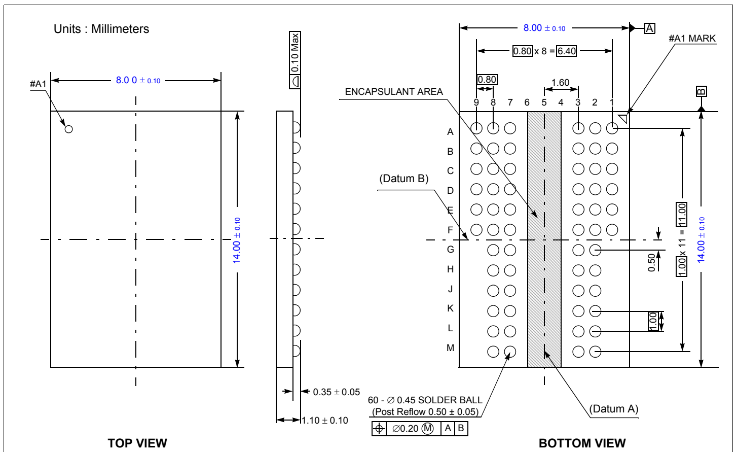
66Ball FBGA Package Dimension
