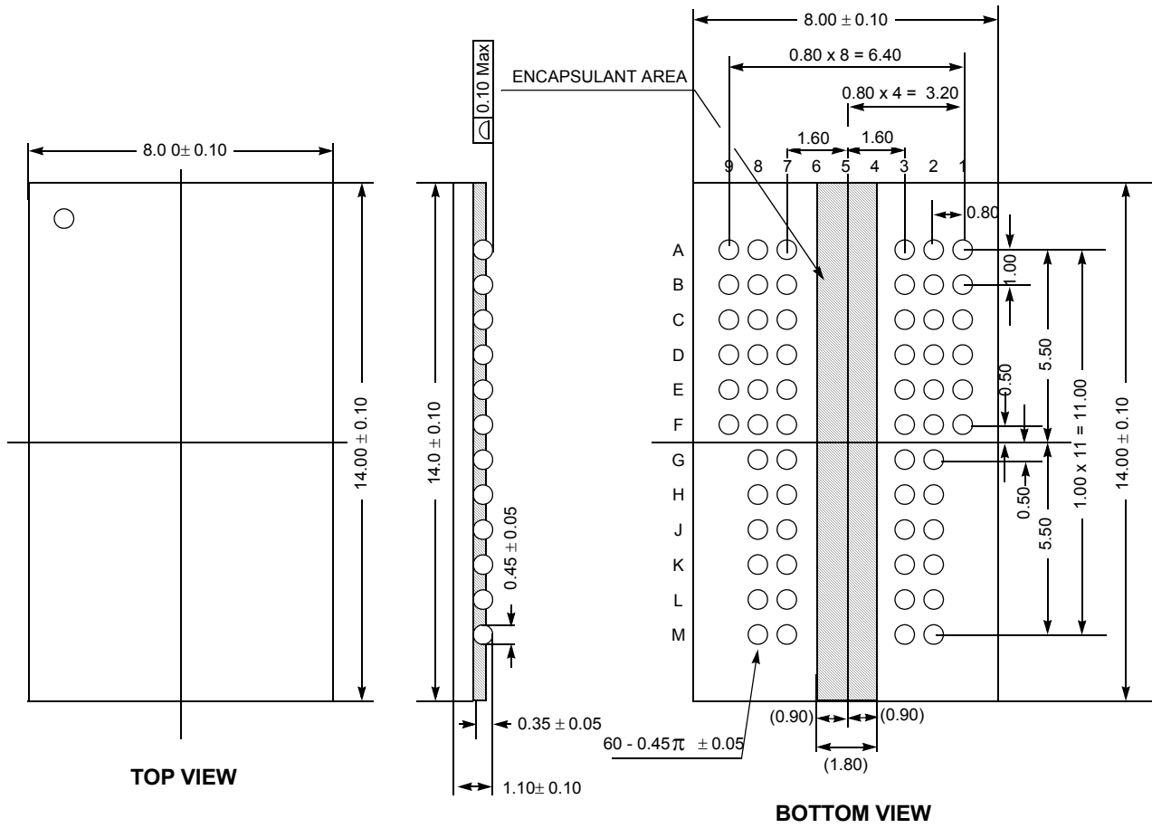
60Ball FBGA 256Mb Package Dimension
