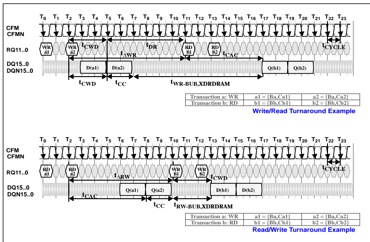
Figure 12 : Write/Read Interaction
