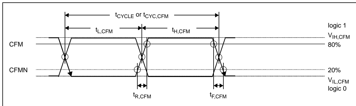
Figure 57 : Clocking Waveforms
