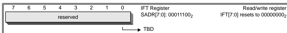
Figure 40 : IFT Register
