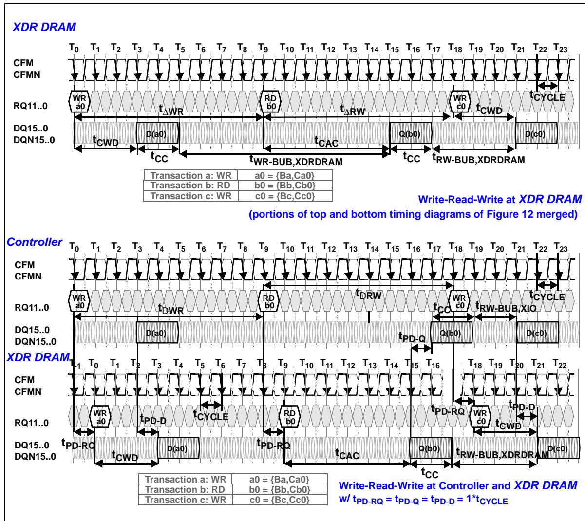
Figure 13 : Propagation Delay
