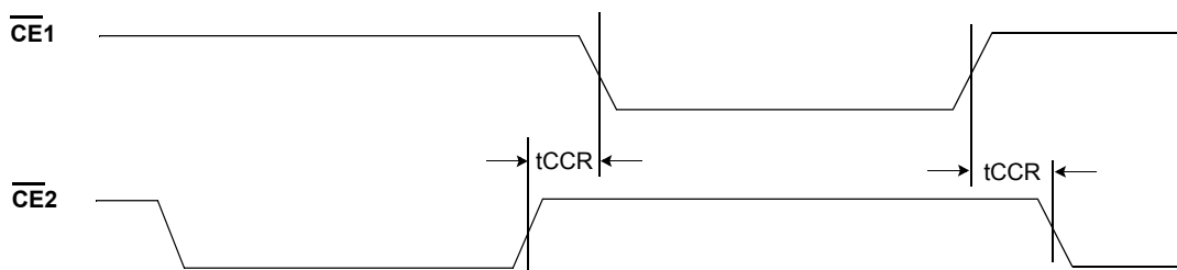
Figure 23. Timings for Alternating Between CE1 and CE2 Control
