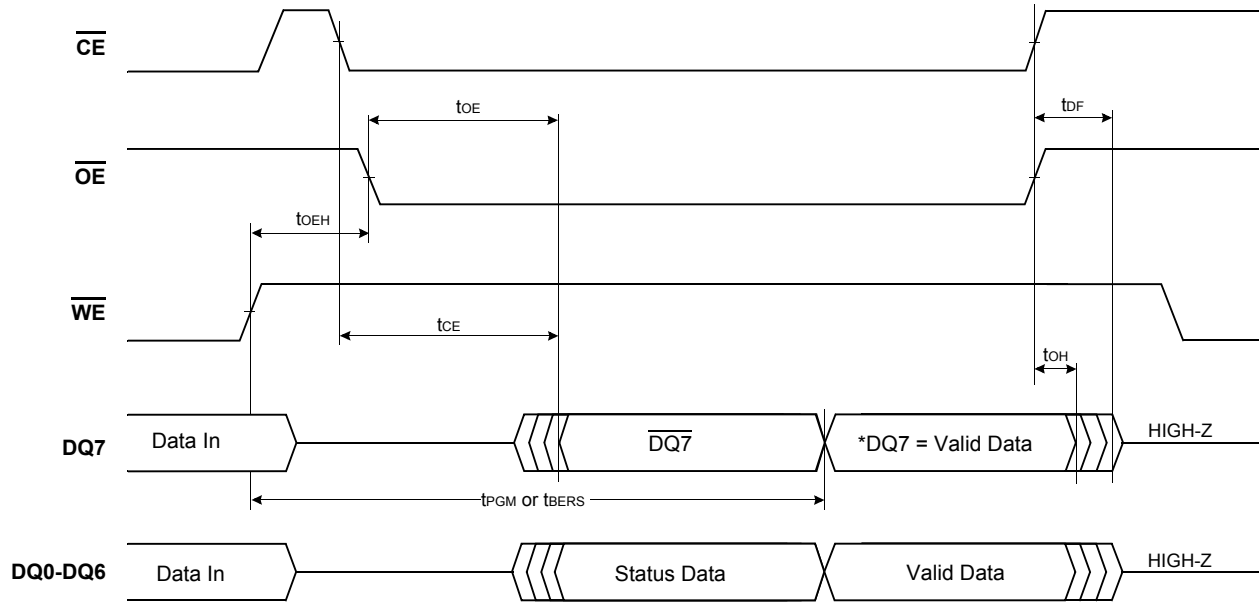
Note : *DQ7=Valid Data (The device has completed the internal operation).
