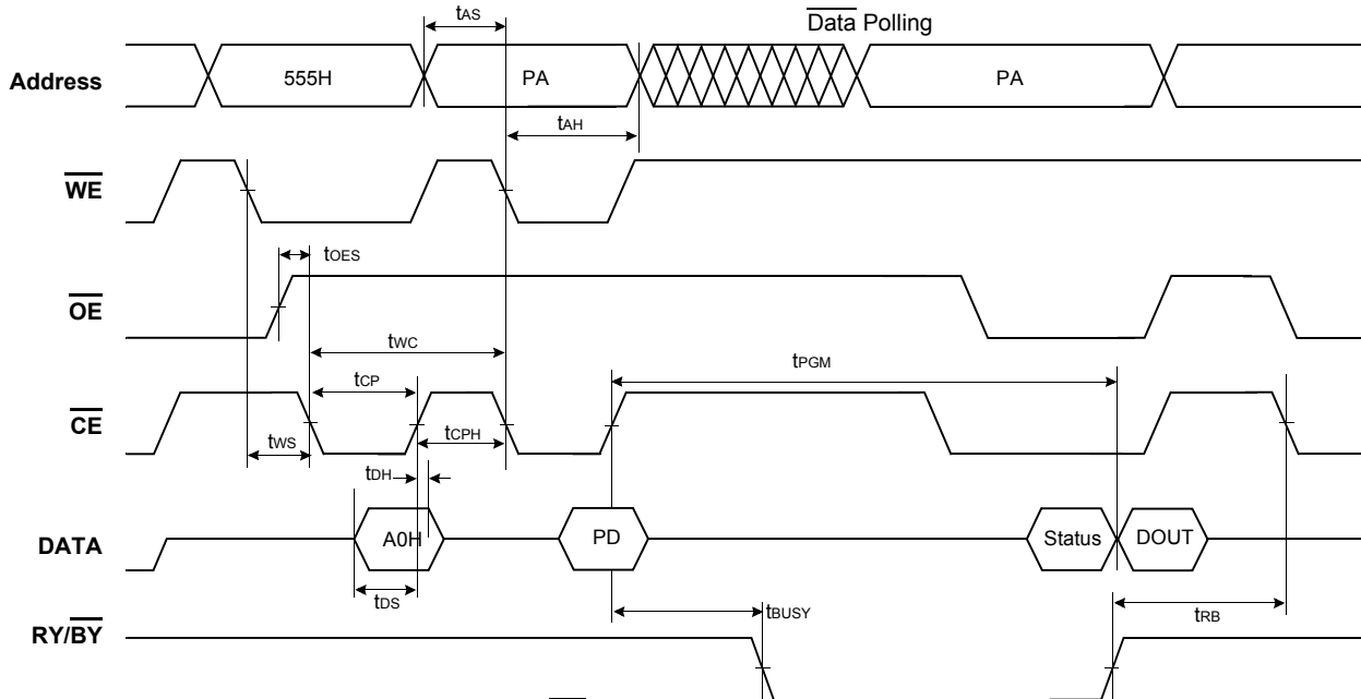
Figure 14. Alternate \overline{CE} Controlled Program Operation Timings
