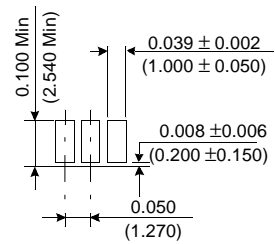
Detail C
