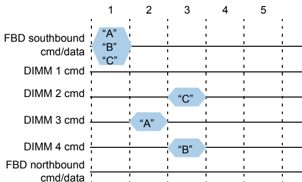
Figure 6. FBDIMM Command Delivery Rules
