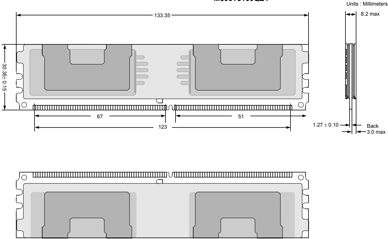
Figure 19 : FBDIMM Physical Dimension -2 (For Heat Spreader): 256Mbx4 based 512Mx72 Module (2Rank) M395T5160QZ4
