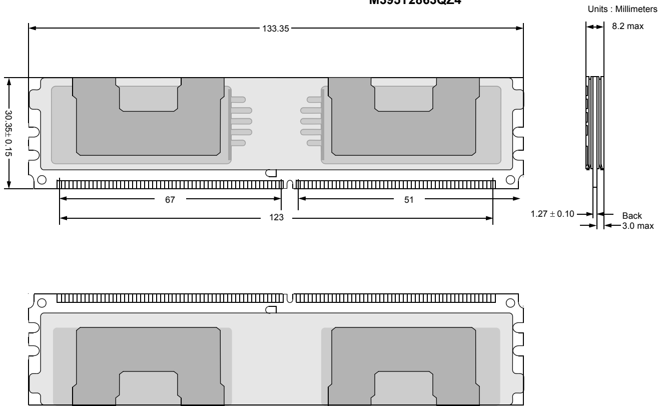
Figure 15 : FBDIMM Physical Dimension -2 (For Heat Spreader): 128Mbx8 based 128Mx72 Module (1Rank) M395T2863QZ4
