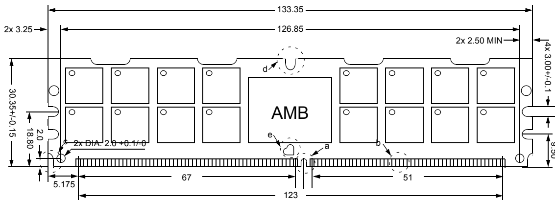
Figure 20 : FBDIMM Physical Dimension -1 (For PCB) : 128Mbx8 based 512Mx72 Module (4Rank) M395T5163QZ4
