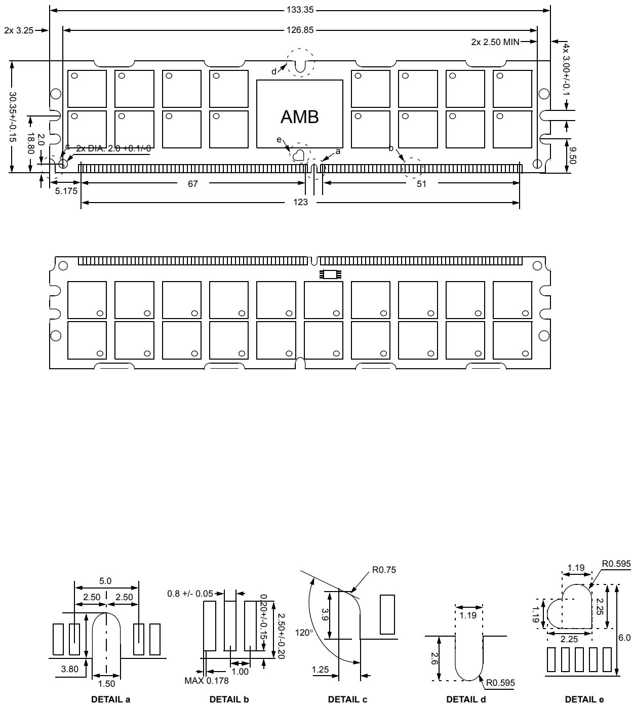
Figure 22 : FBDIMM Physical Dimension -1 (For PCB) : 256Mbx4 based 1Gx72 Module (4Rank) M395T1G60QJ4
