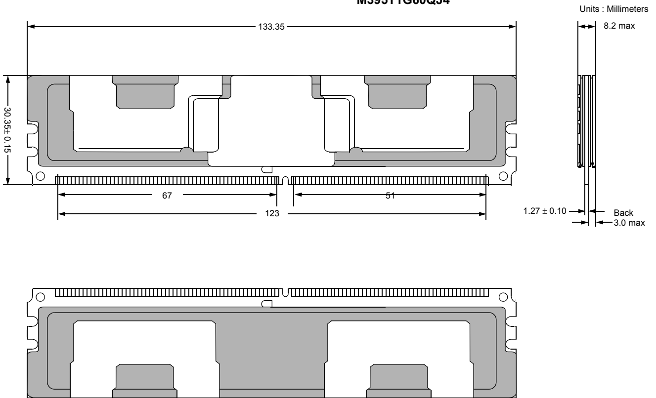
Figure 23 : FBDIMM Physical Dimension -2 (For Heat Spreader): 256Mbx4 based 1Gx72 Module (4Rank) M395T1G60QJ4
