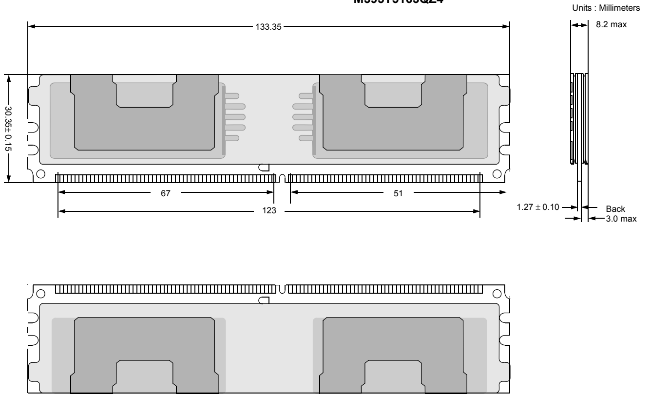
Figure 21 : FBDIMM Physical Dimension -2 (For Heat Spreader): 128Mbx8 based 512Mx72 Module (4Rank) M395T5163QZ4
