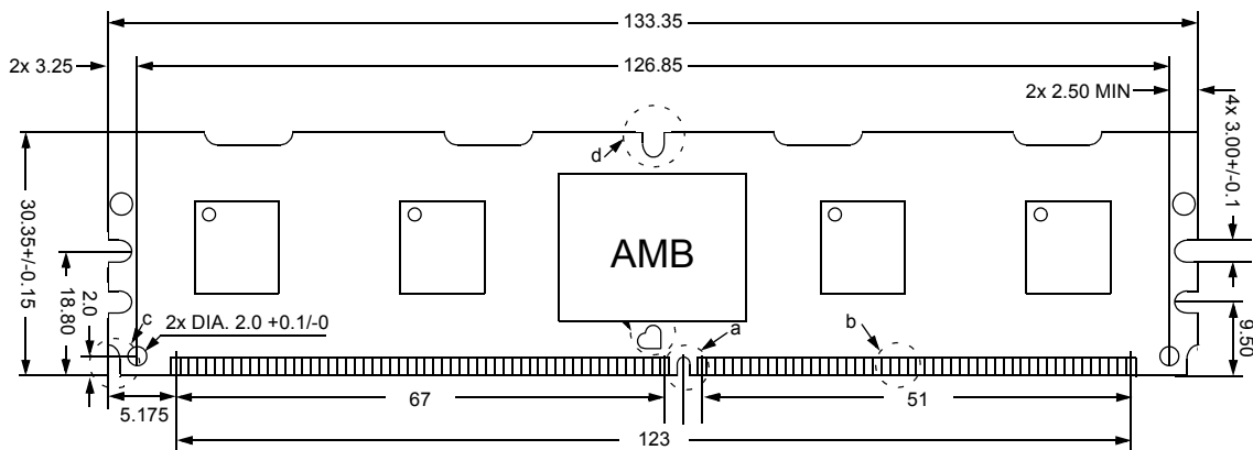
Figure 14 : FBDIMM Physical Dimension -1 (For PCB) : 128Mbx8 based 128Mx72 Module (1Rank) M395T2863QZ4
