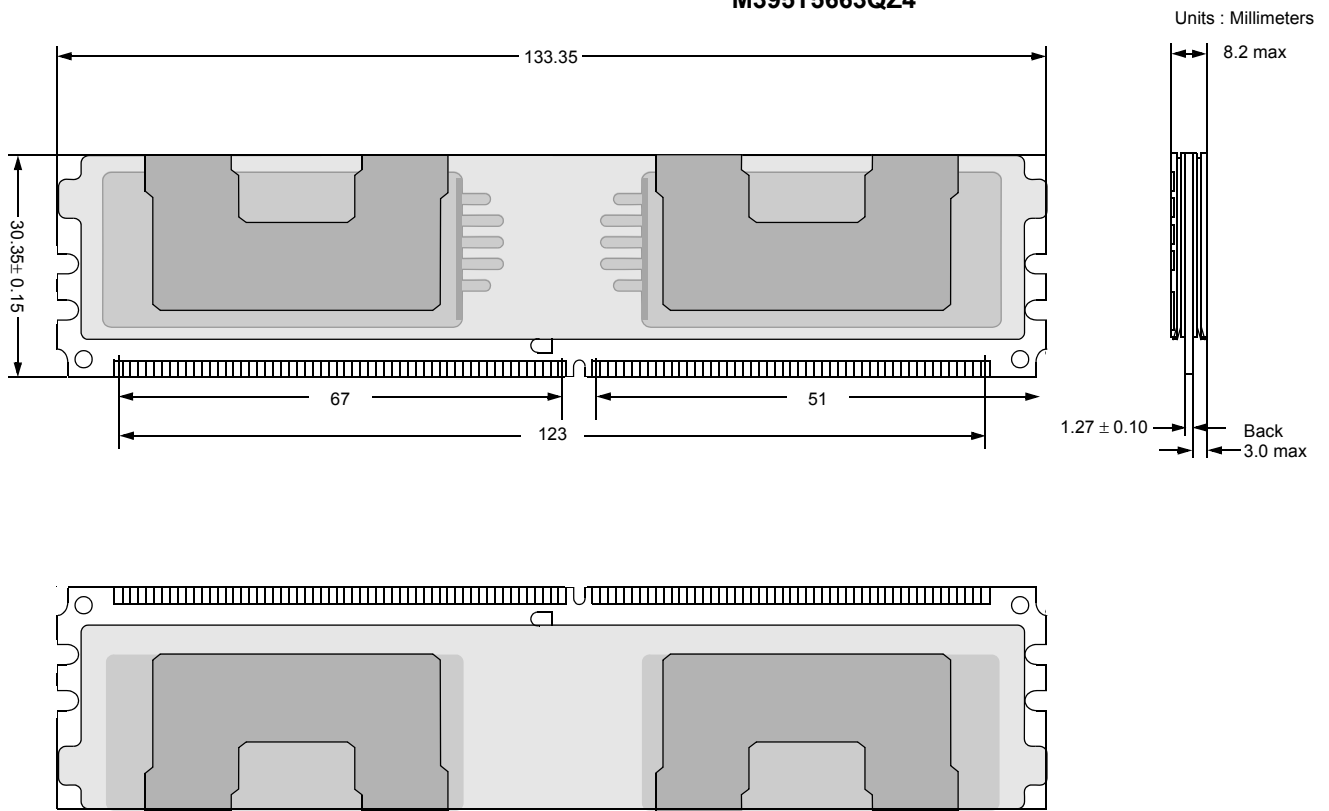
Figure 17 : FBDIMM Physical Dimension -2 (For Heat Spreader) : 128Mbx8 based 256Mx72 Module (2Rank) M395T5663QZ4
