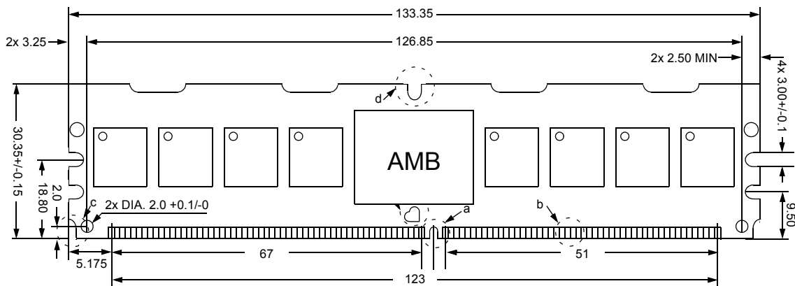
Figure 16 : FBDIMM Physical Dimension -1 (For PCB) : 128Mbx8 based 256Mx72 Module (2Rank) M395T5663QZ4
