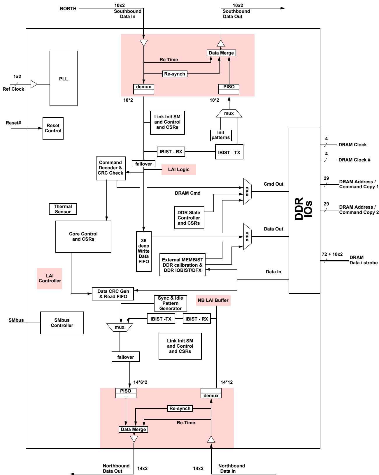
Figure 11. Advanced Memory Buffer Block Diagram
