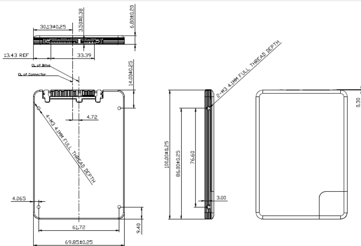
Figure 2-1. Physical dimension
